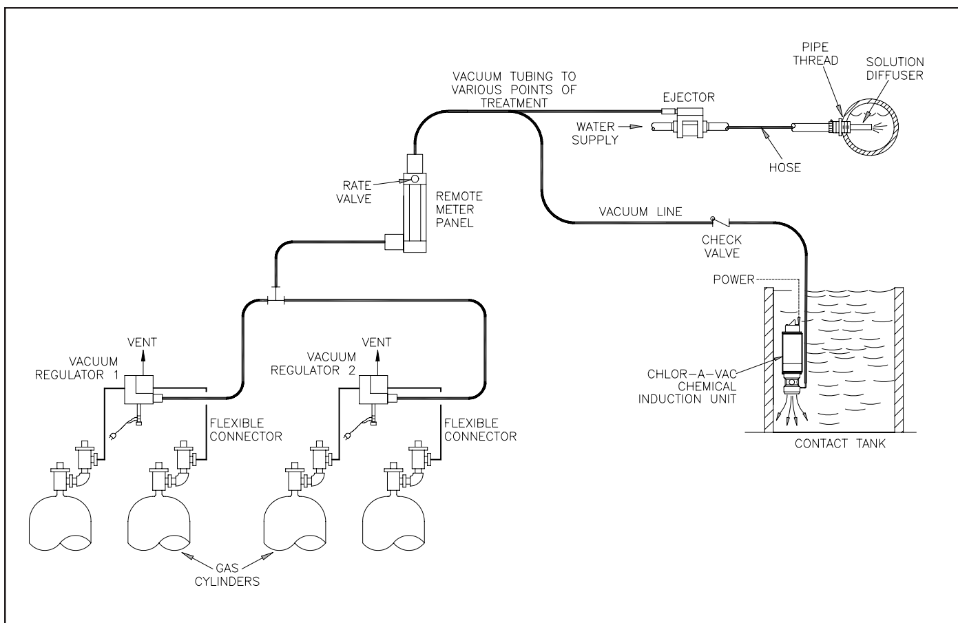
Figure 6 - Manifold Mounted Automatic Switchover
