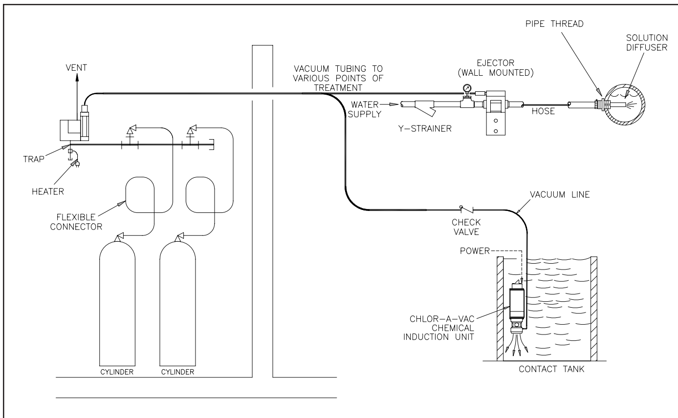
Figure 3 - Vertical Manifold Mounted
