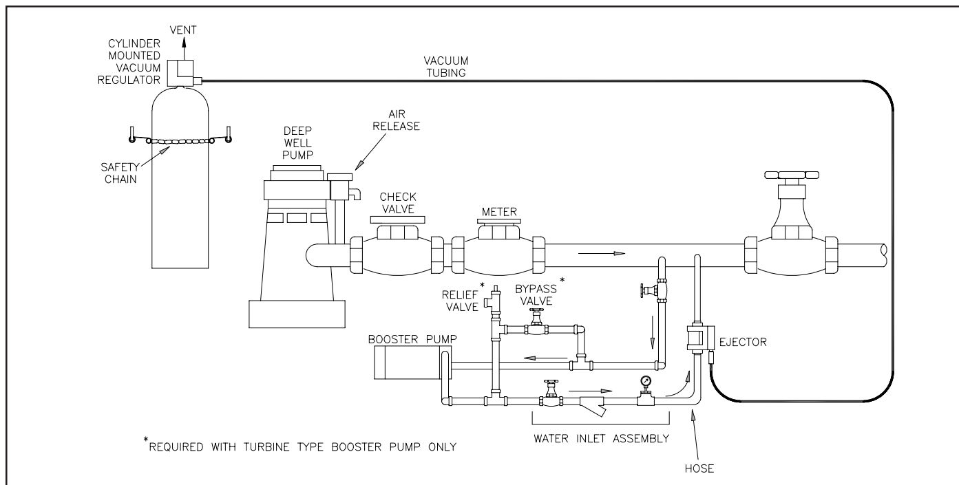
Figure 2 - Cylinder Mounted Deep Well
