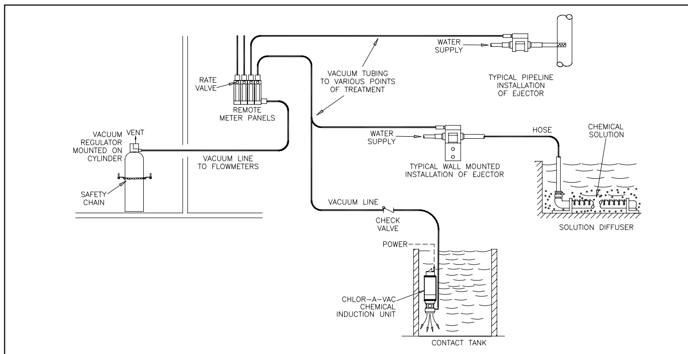
Figure 1 - Multiple, Remote Metering Arrangement
