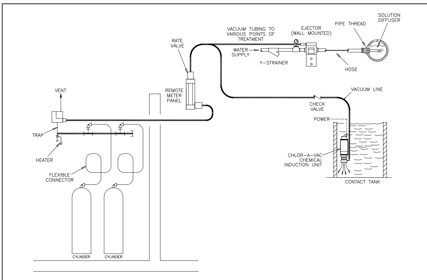
Figure 4 - Horizontal Manifold Mounted
