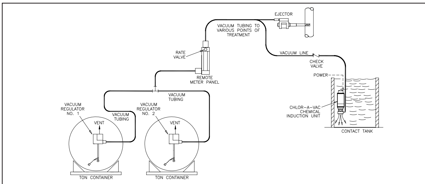
Figure 8 - Ton Container Mounted Automatic Switchover
