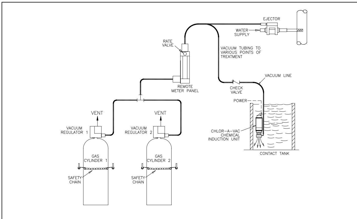
Figure 5 - Direct Cylinder Mounted Automatic Switchover
